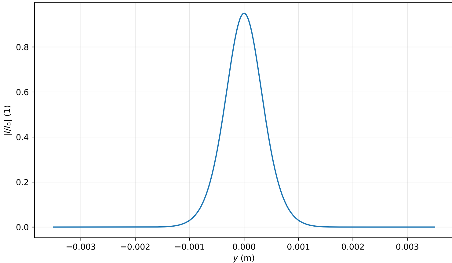
Intensity profile I(x=0, y, z=1.194)/I_0 , P_{in}=0.4P_{cr} , artificial time
